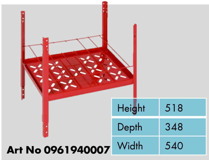
Shelf for 500ml
