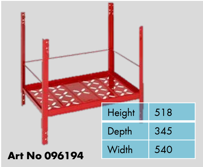
Shelf for 1000ml
