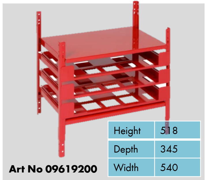
Drawer Component for 3 unit of ORSY 200 cases
